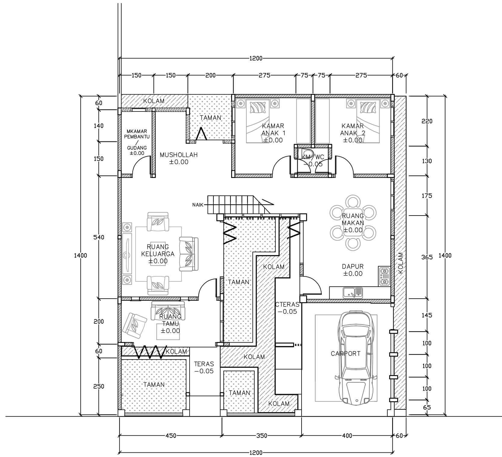
DENAH LANTAI 1 SKALA 1 : 100
