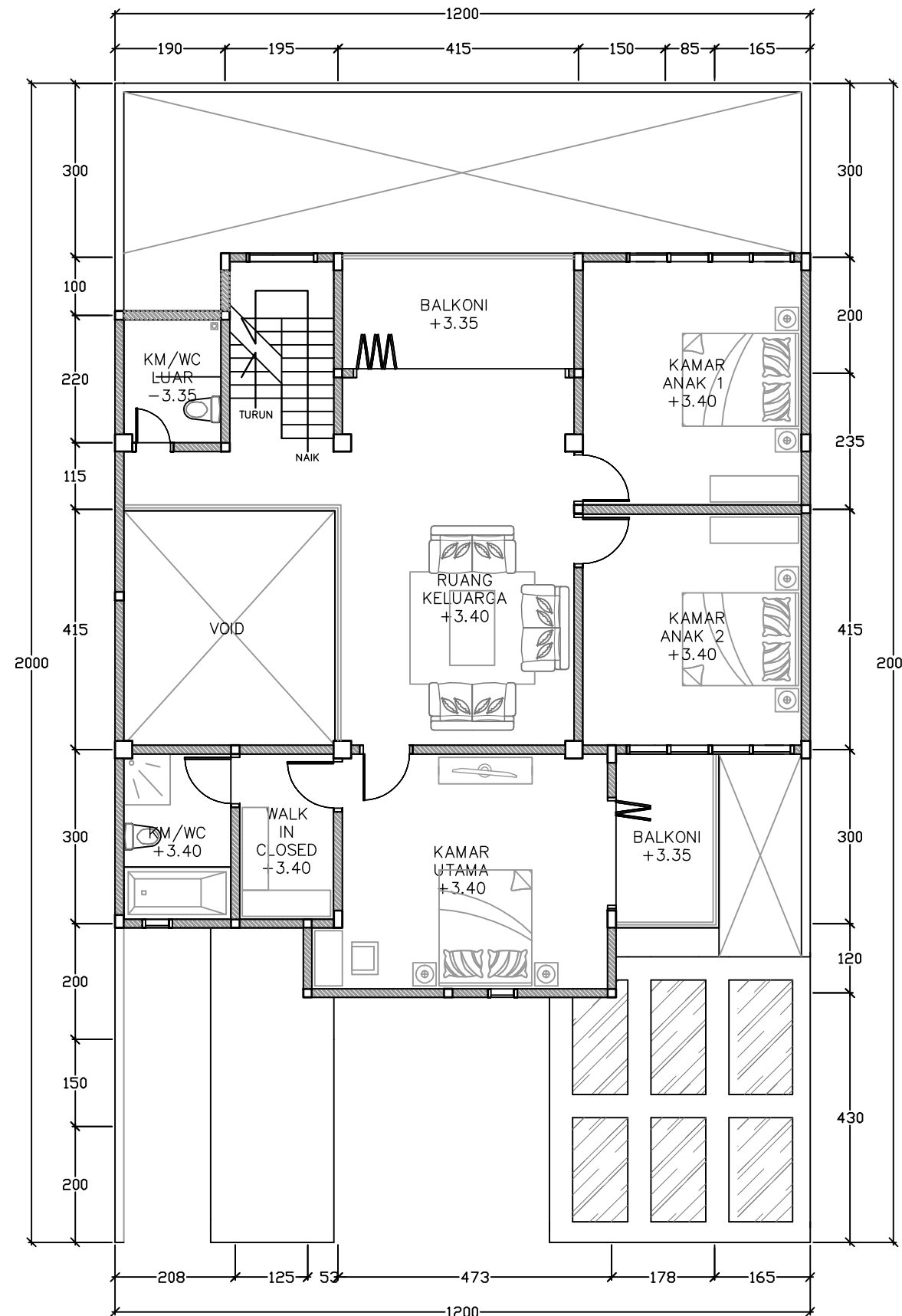
DENAH LANTAI 2 SKALA 1 : 100
