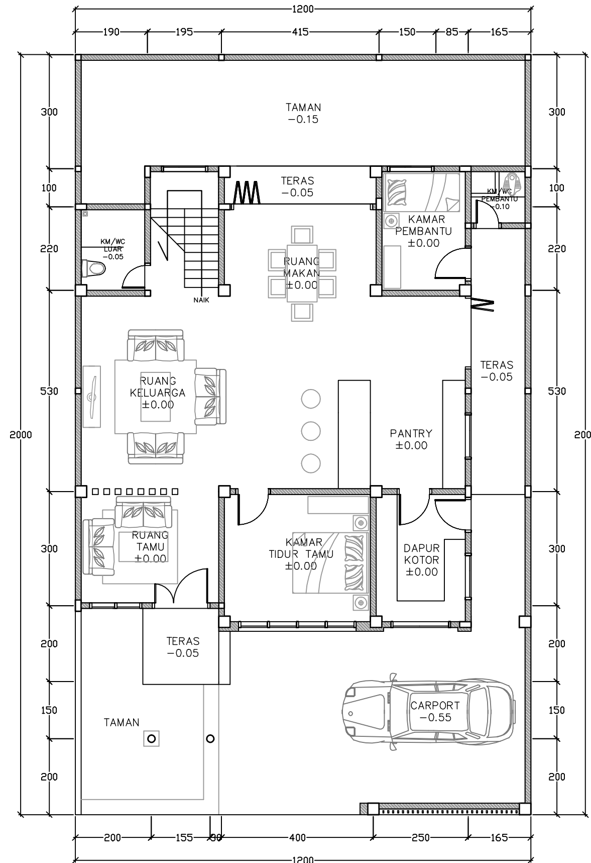
DENAH LANTAI 1 SKALA 1 : 100
