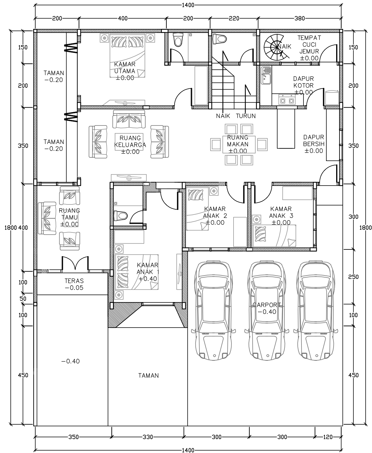
DENAH LANTAI 1
