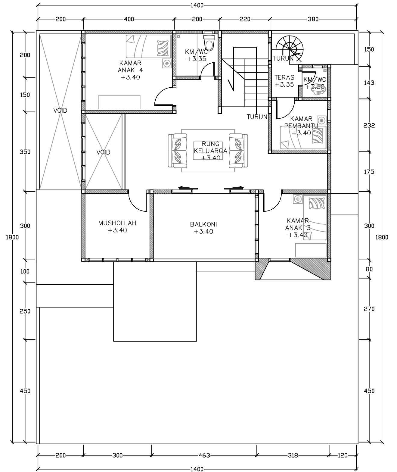
DENAH LANTAI 2
