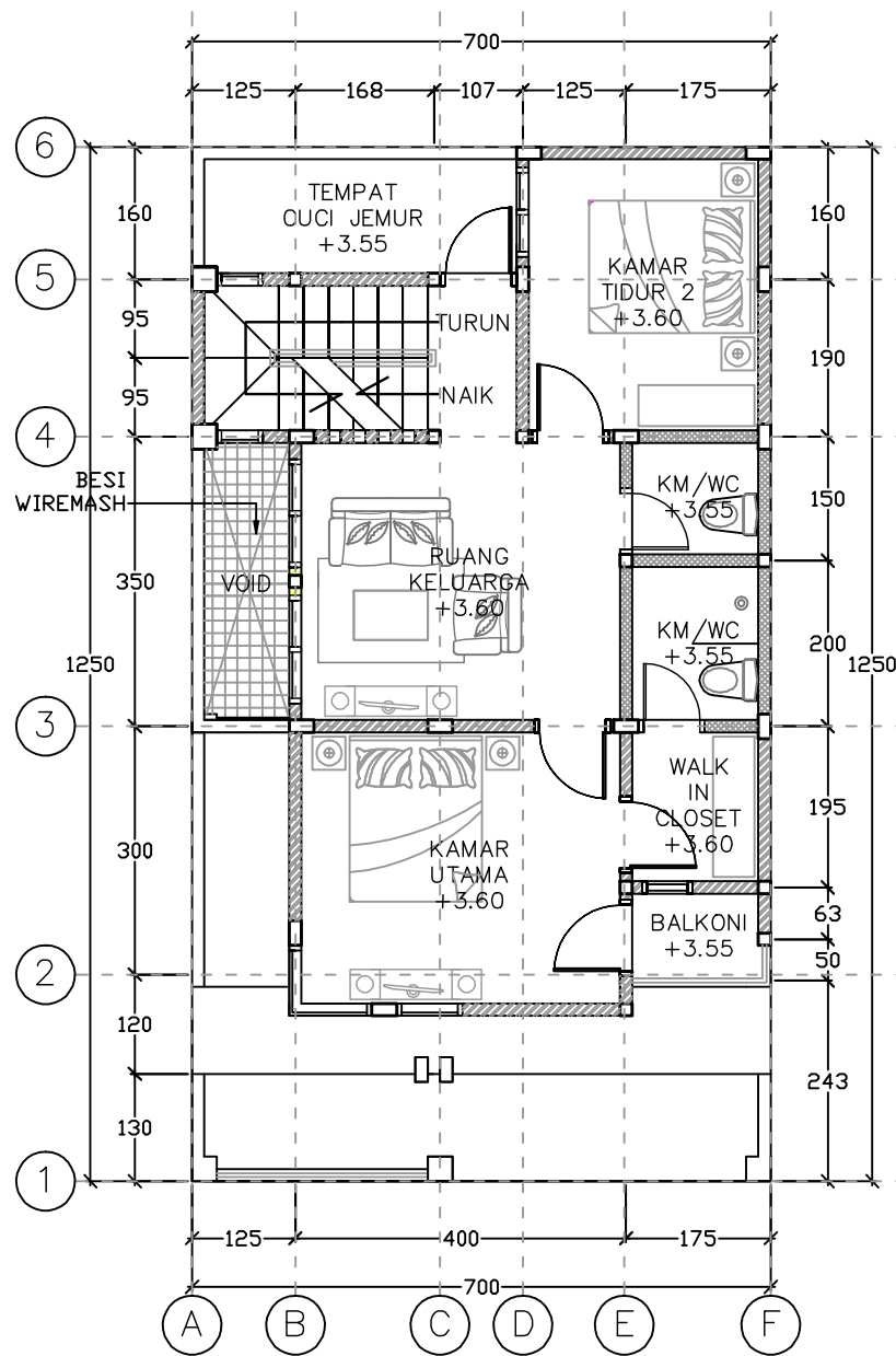
DENAH LANTAI 2
