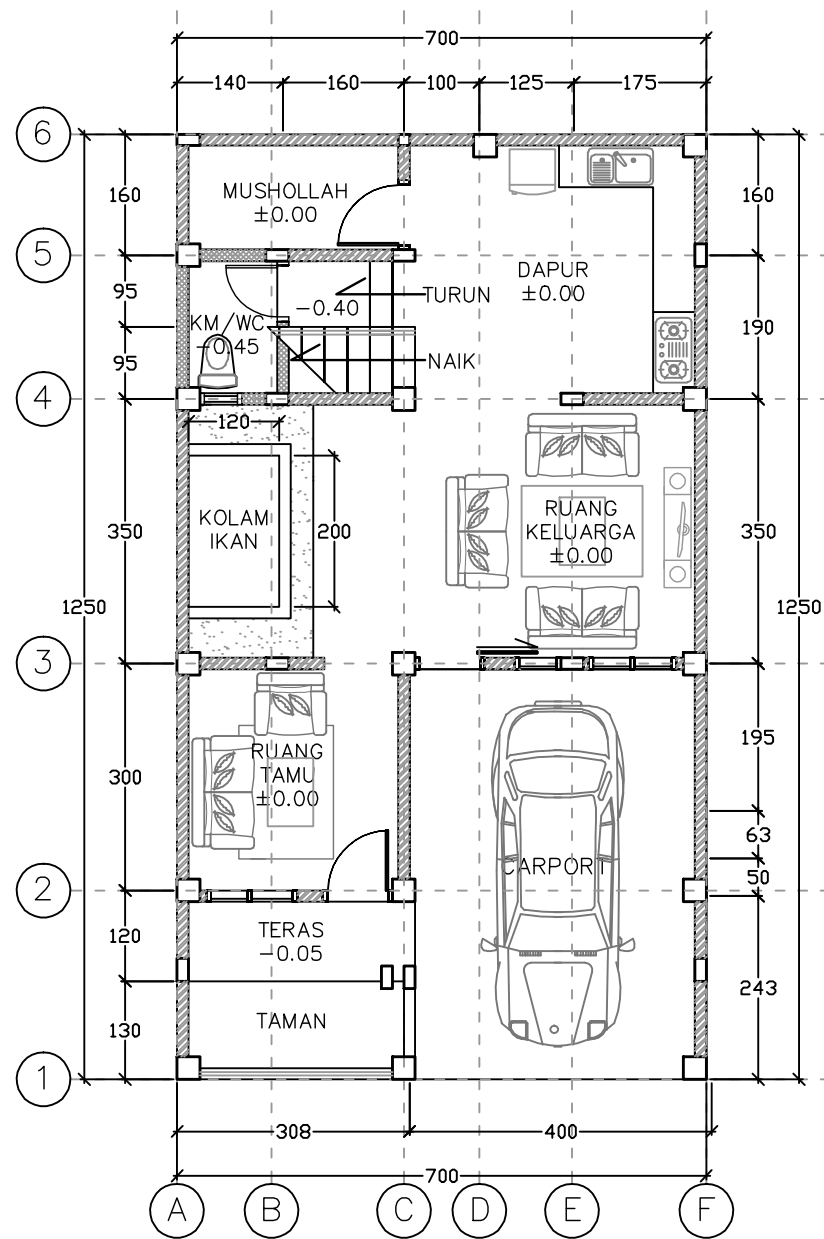
DENAH LANTAI 1
