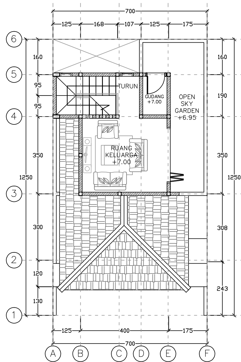
DENAH LANTAI 3
