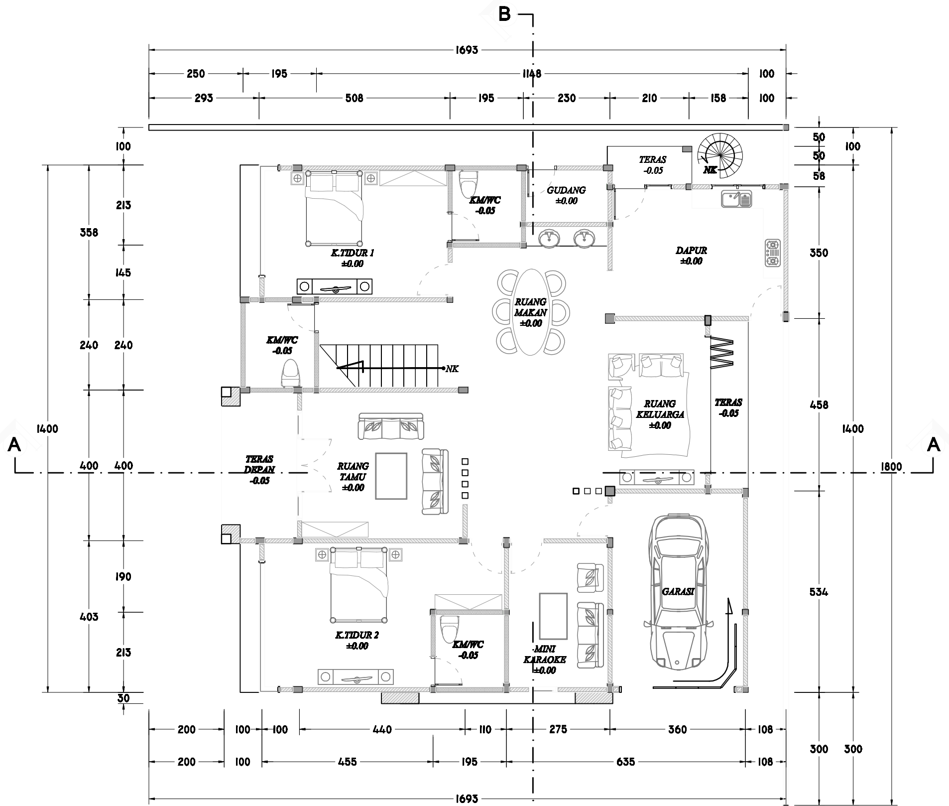
DENAH LANTAI 1 SKALA 1:100
